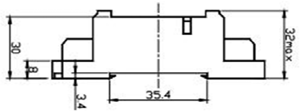
Socket With Finger Safe Terminals
