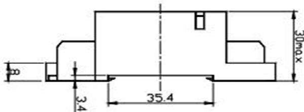
Socket Without Finger Safe Terminals
